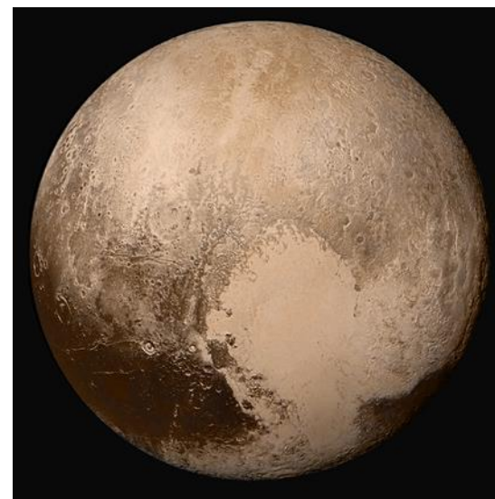
Plutone
