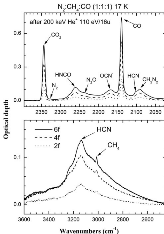
FIG. 2. Spectra after 200 keV He + irradiation of the ice mixtures for the three considered thicknesses.
